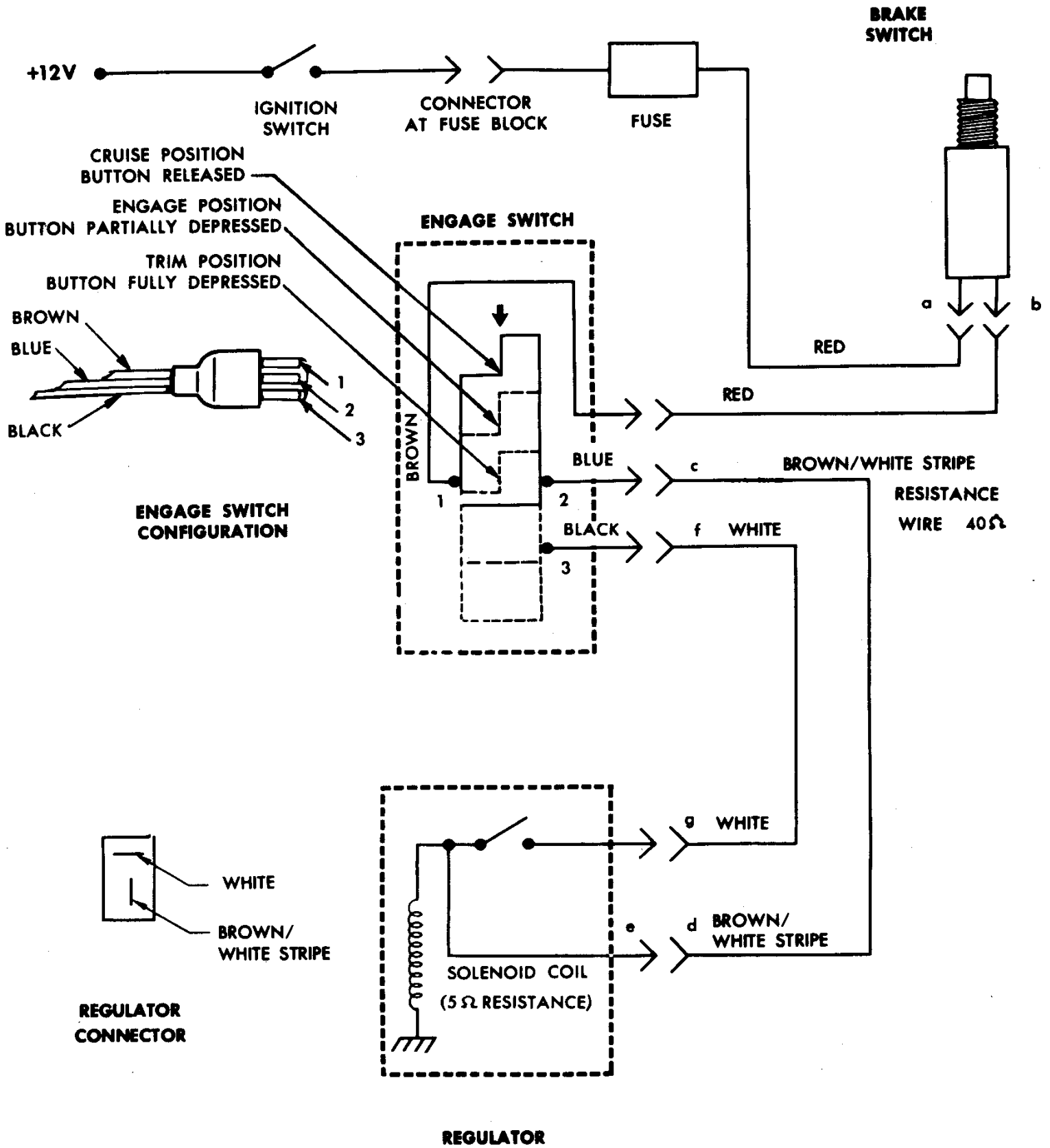
1970-73 Camaro Cruise Master Wiring Circuit
