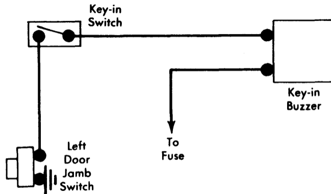
GENERAL MOTORS CHEVROLET BUZZER WIRING DIAGRAM
